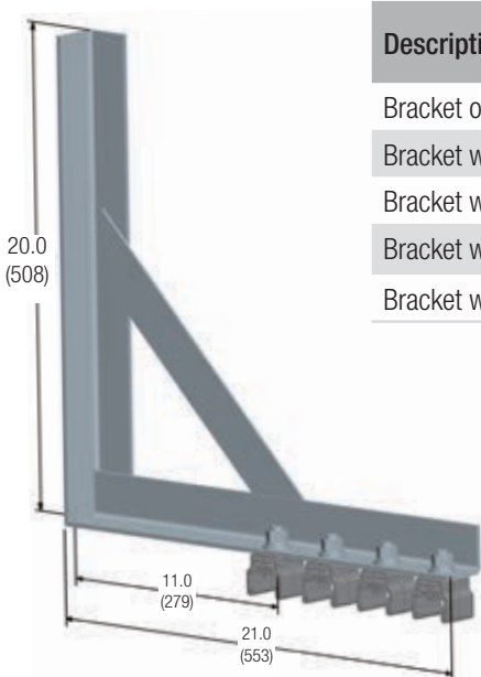
Braced Web (25691)
