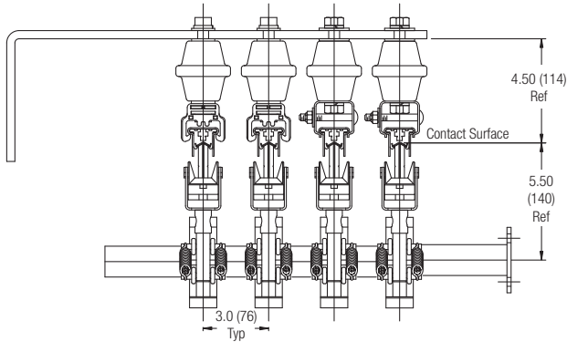
500A - with Insulators
